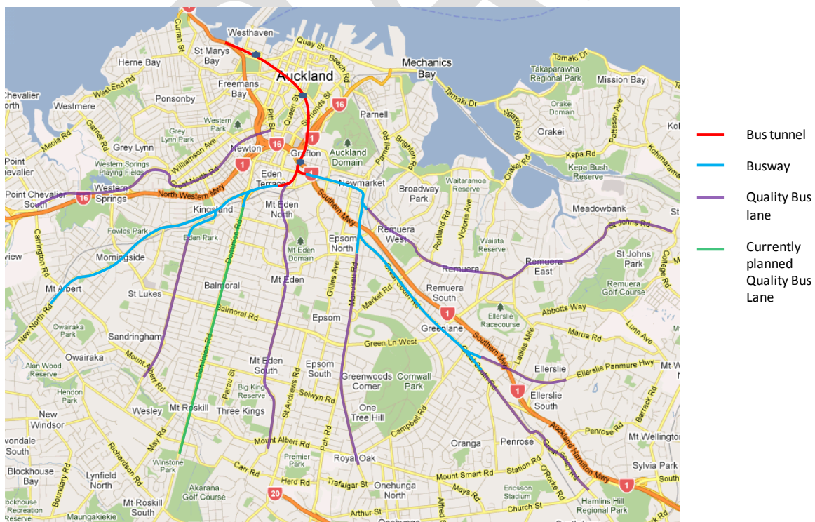
Figure 3-4: Required Wider Network Infrastructure to Support Bus Rapid Transit
