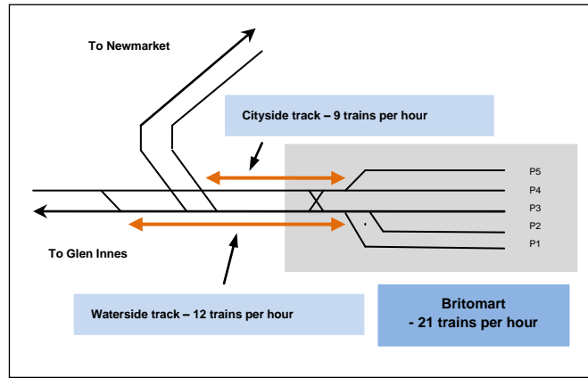
Figure 3-2 Current Arrangement of Britomart Approach Tracks and Platforms
