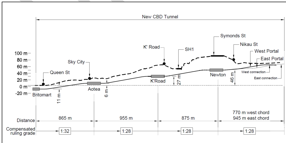
Figure 4-2 Proposed CBD Rail Link Long Section and Gradient Profile
