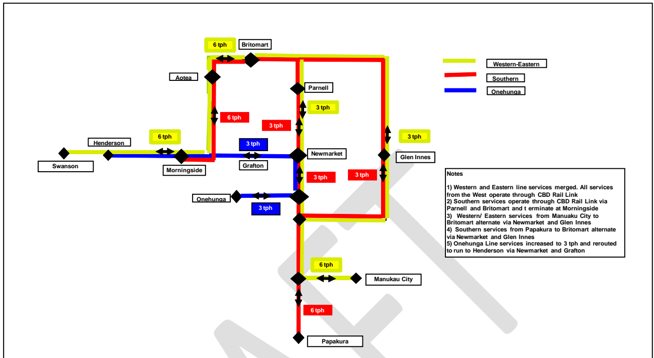
Figure 4-6 Minimum Rolling Stock- Initial Electric Train Services
