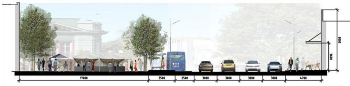
Figure 5-19 Indicative section at the corner of Mt Eden Road and Symonds Street; indicating potential for public transport interchanges and amenity / community space integrated with existing environment and proposed Newton Station.
